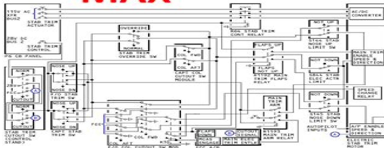
Horizontal Stabilizer Trim Control System - Functional Description - Electric Trim
