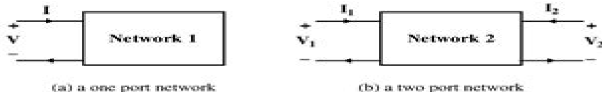
Figure 7.1: Diagram defining network ports.
