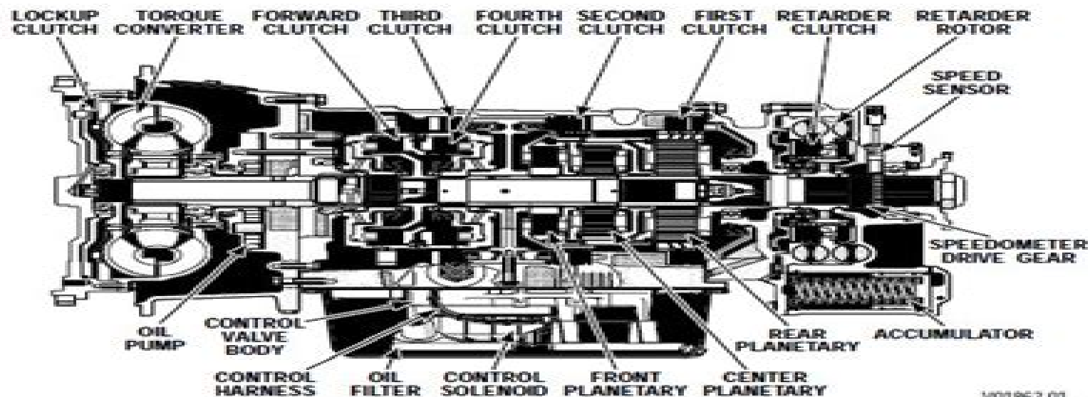
Cross Section of HTB 748
