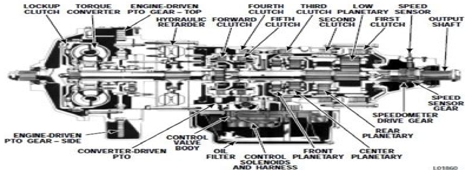
Cross Section of CLBT 755
