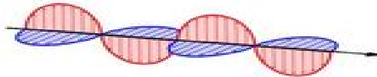
Electromagnetic Wave
