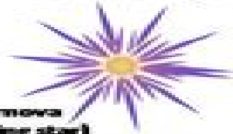
Gamma Rays
