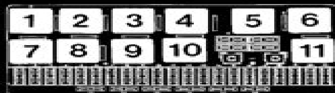
Fuse/Relay Panel
