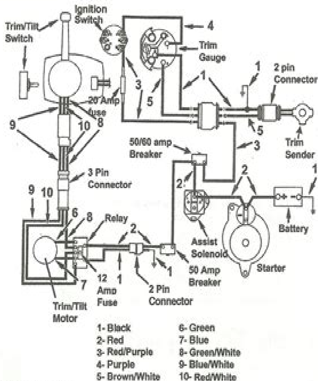
Fig. 102 Power trim/tilt—1993-95 Ford models
