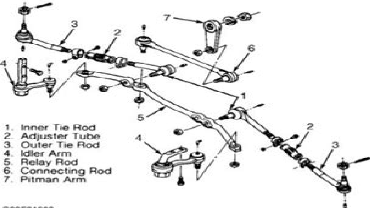
Fig. 2: Exploded View Of Steering Linkage (Astro & Safari - 2WD) Courtesy of GENERAL MOTORS CORP.
