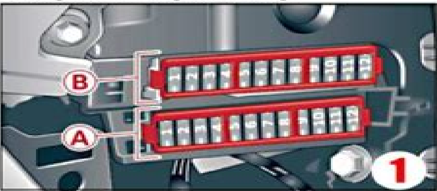
Front passenger's side of the cockpit fuse panel with plastic clip
