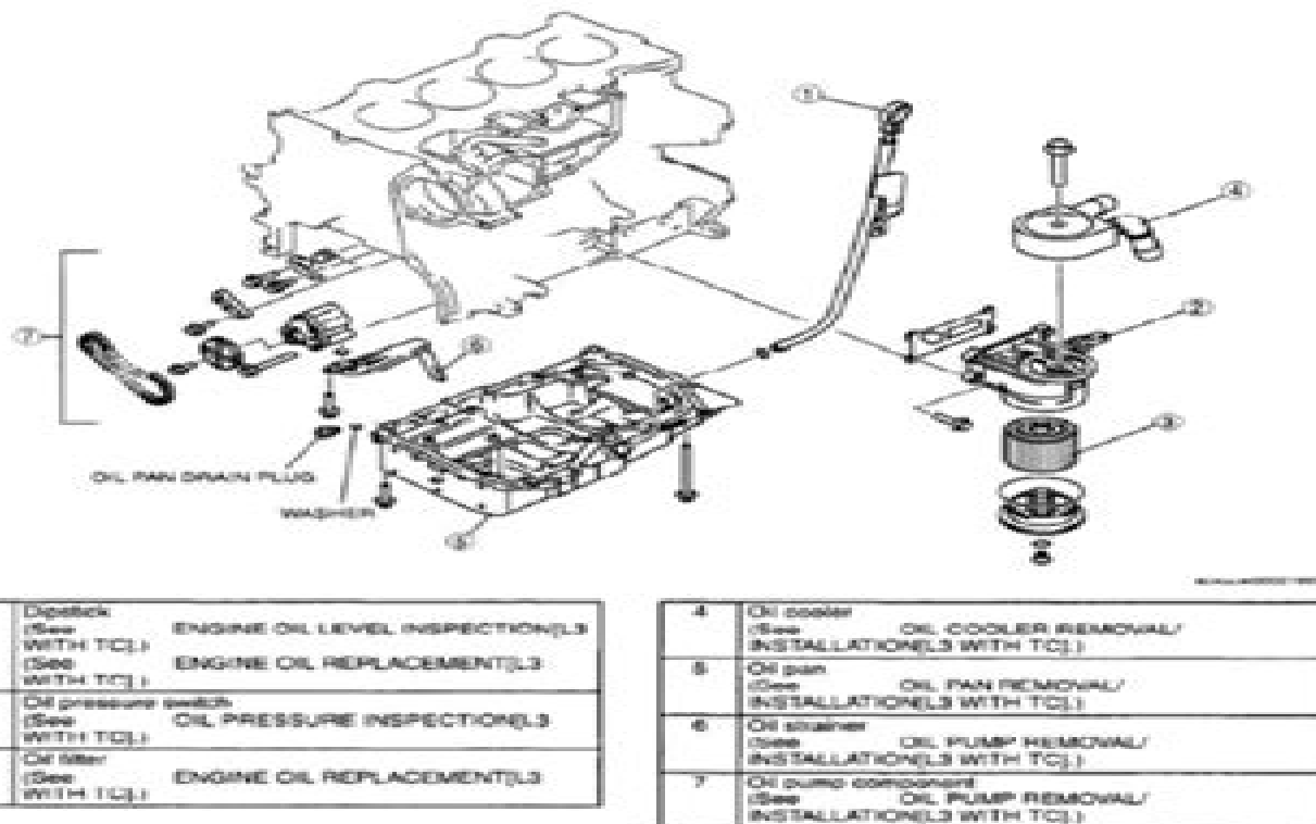
Fig. 1: Identifying Lubrication System Components [L3 With TC]
