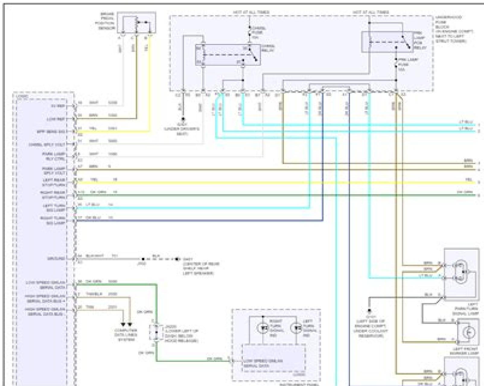
Fig 2: Exterior Lamps Circuit (1 of 2)
