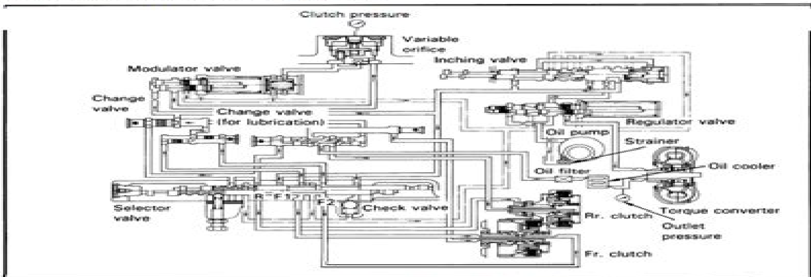
Hydraulic Circuit Diagram (Two-Speed) Option
