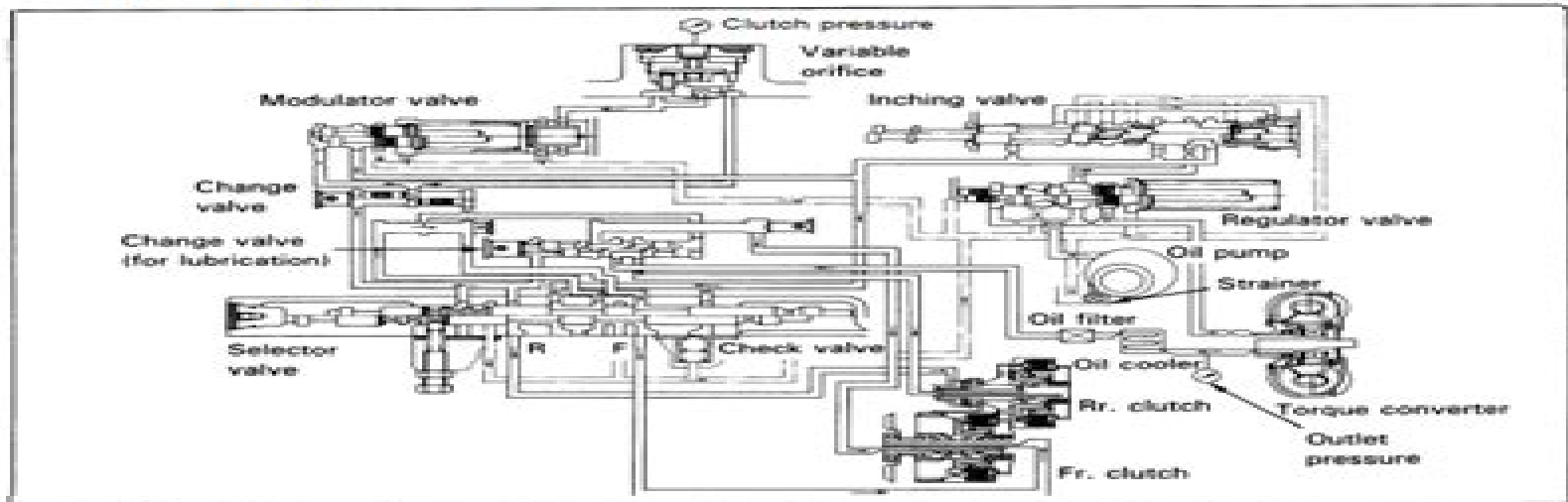
Hydraulic Circuit Diagram (One-Speed)
