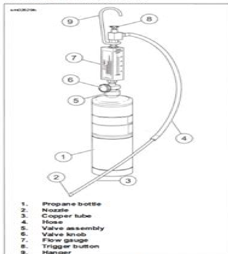
Figure 6-35. Leak Tester
