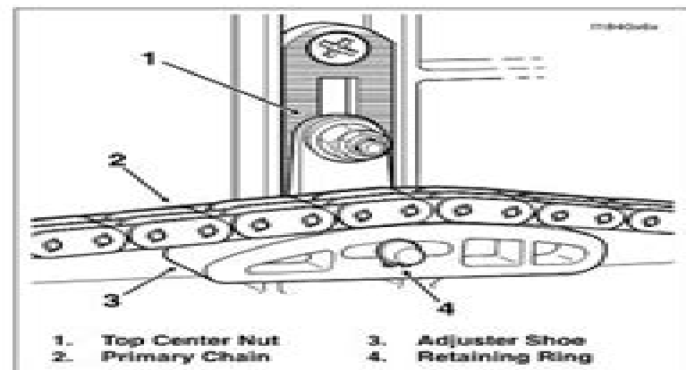
Figure 6-1. Primary Chain Tensioner Assembly
