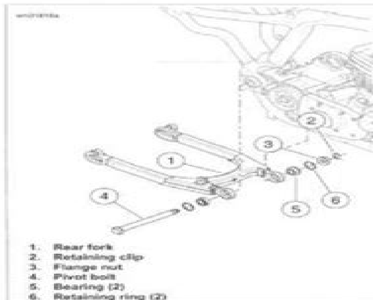
Figure 2-109. Rear Fork Assembly.
