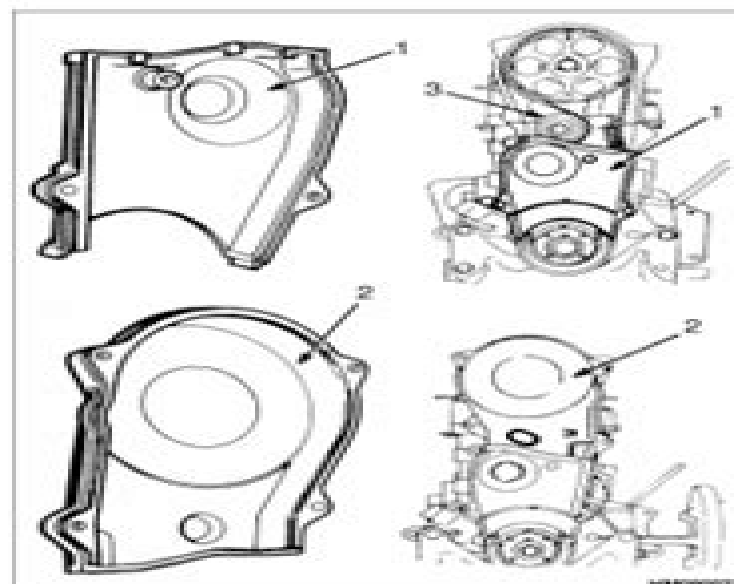
Figure 2. Timing Belt Covers
