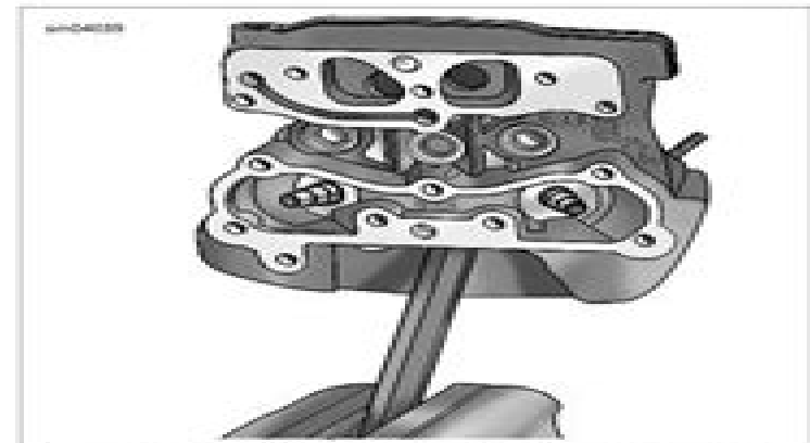
Figure 3-4. Install Cylinder Head Holding Fixture in Vise
