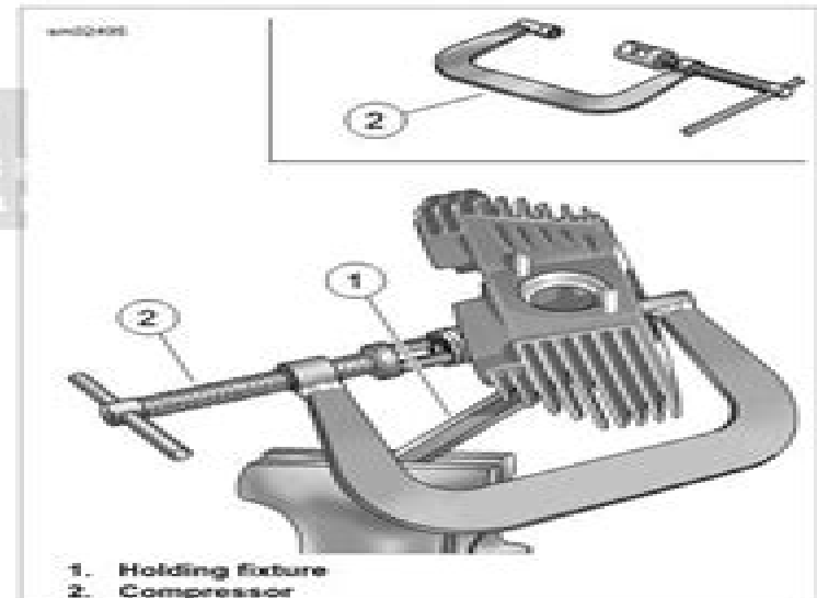
Figure 3-5. Valve Spring Compressor (Part No. HD-34736-B)
