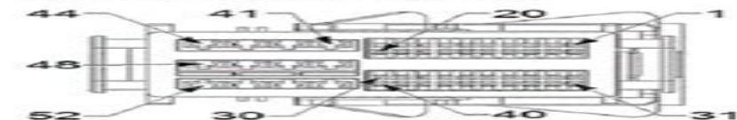
52 pin Dodge, Jeep, Chrysler Head Unit connector.
