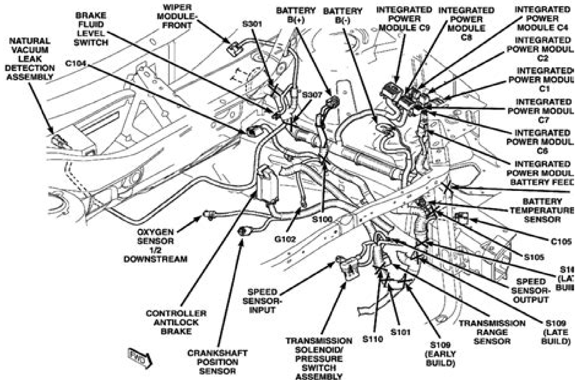
ENGINE COMPARTMENT - LEFT FRONT
