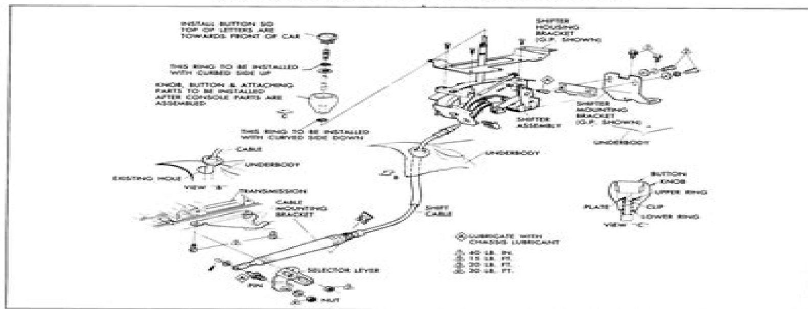
Fig. 7E-34 Console Shift Controls - Tempest and Grand Prix
