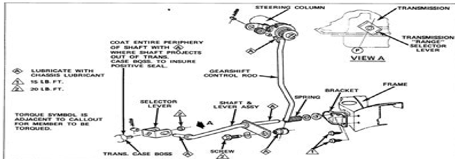
Fig. 7E-33 Column Shift Controls - Tempest and Grand Prix
