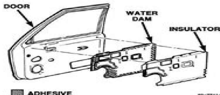
Fig. 14 Waterdam-Insulator
