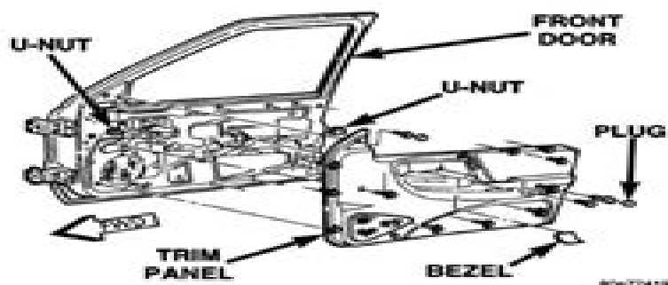
Fig. 13 Front Door Trim Panel
