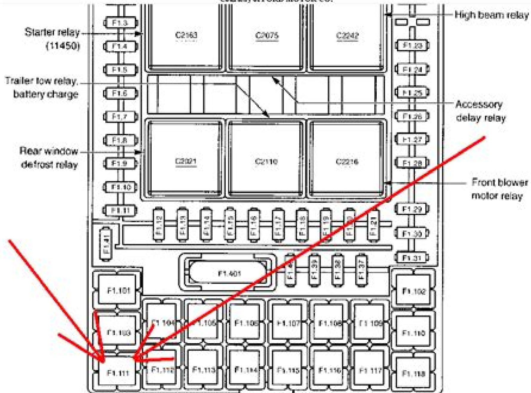
Fig. 2: Identifying Central Junction Box Components
