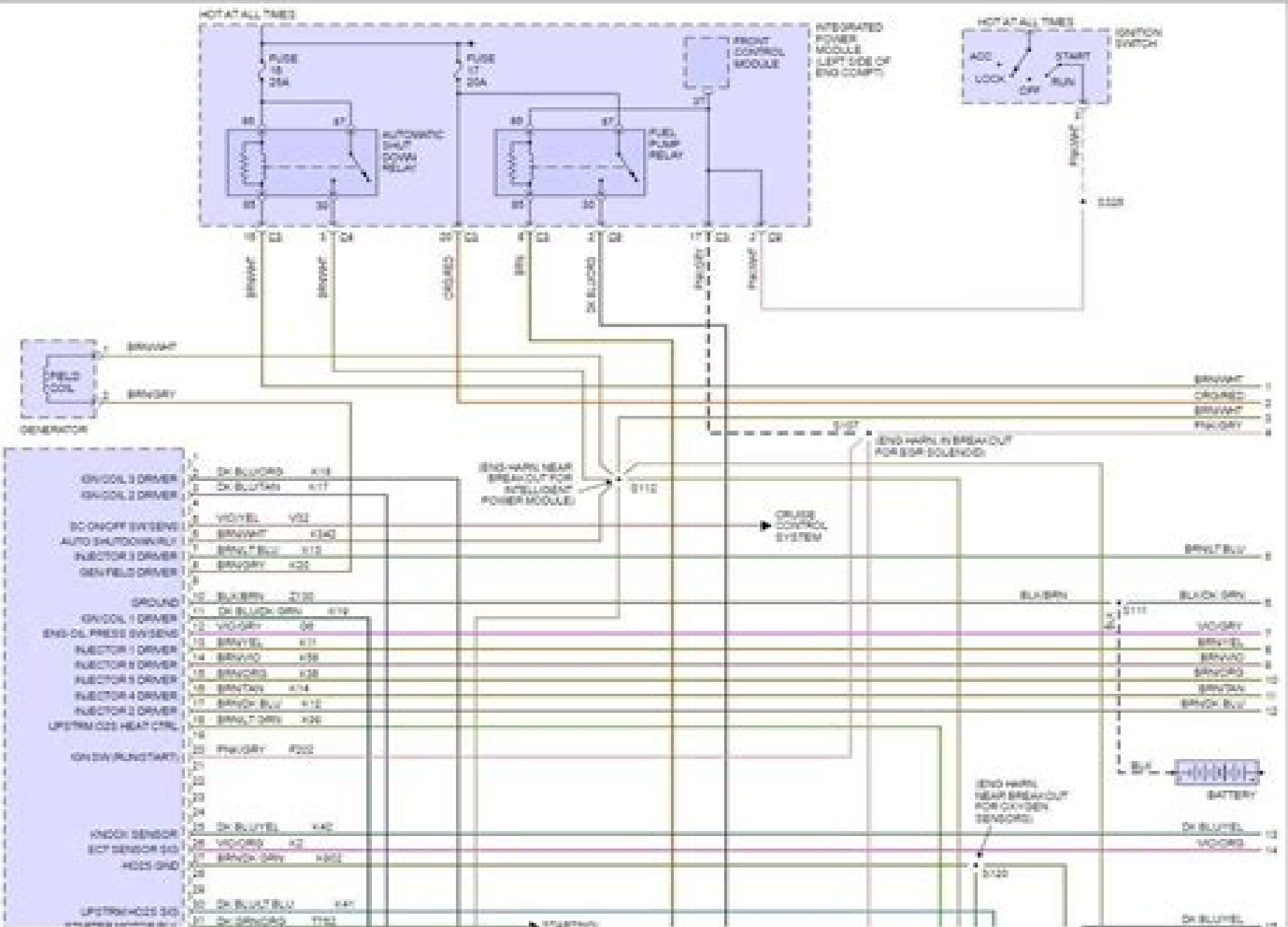
Fig 1: 3.3L Engine Performance Circuits (1 of 3)
