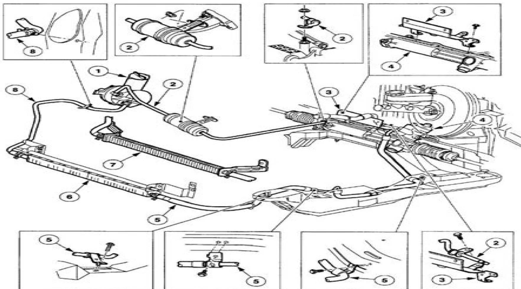
Fig 1: Locating Power Steering Components (3.0L 2V Gasoline Engines - CII Pump)
