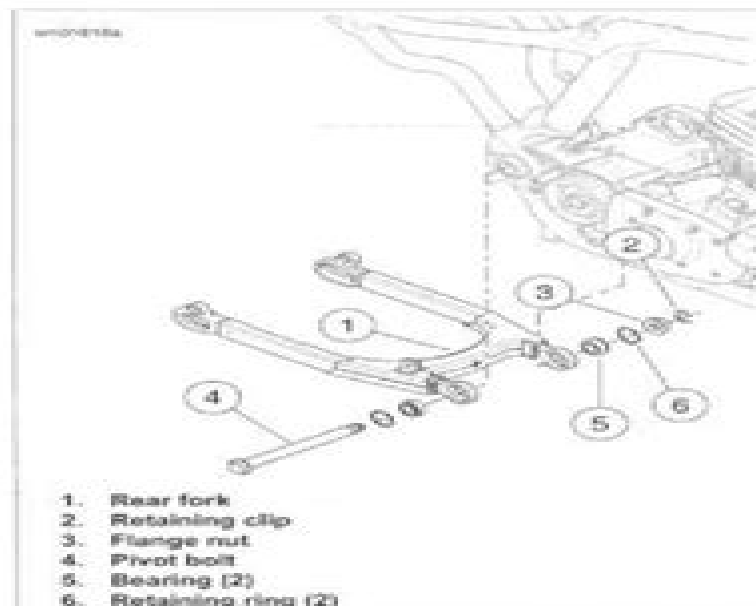
Figure 2-109. Rear Fork Assembly
