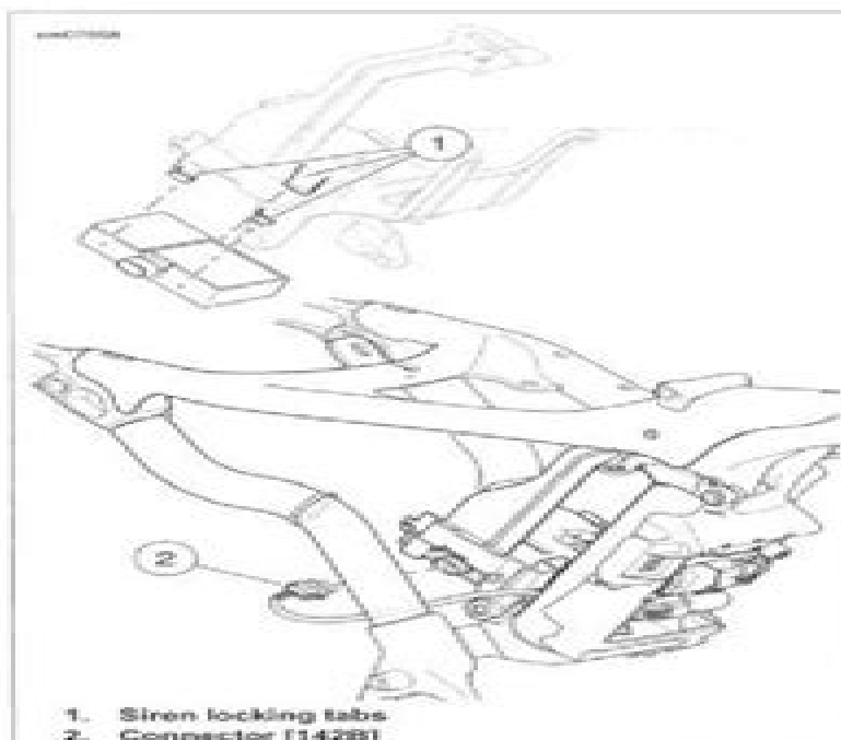
Figure 6-13. Smart Siren
