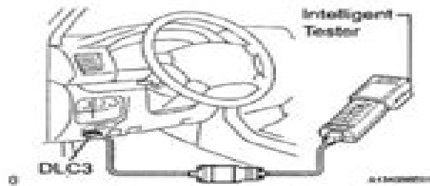
Fig. 2: Connecting Intelligent Tester To DLC3
