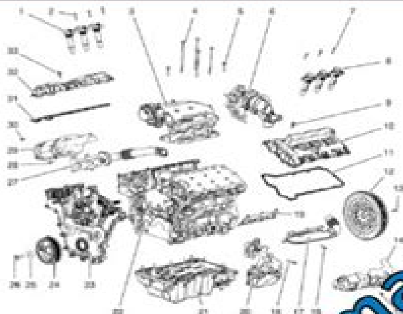
Fig. 1: Disassembled View Of Engine, Cylinder & Component Assembly (LAC) Courtesy of GENERAL MOTORS CORP.
