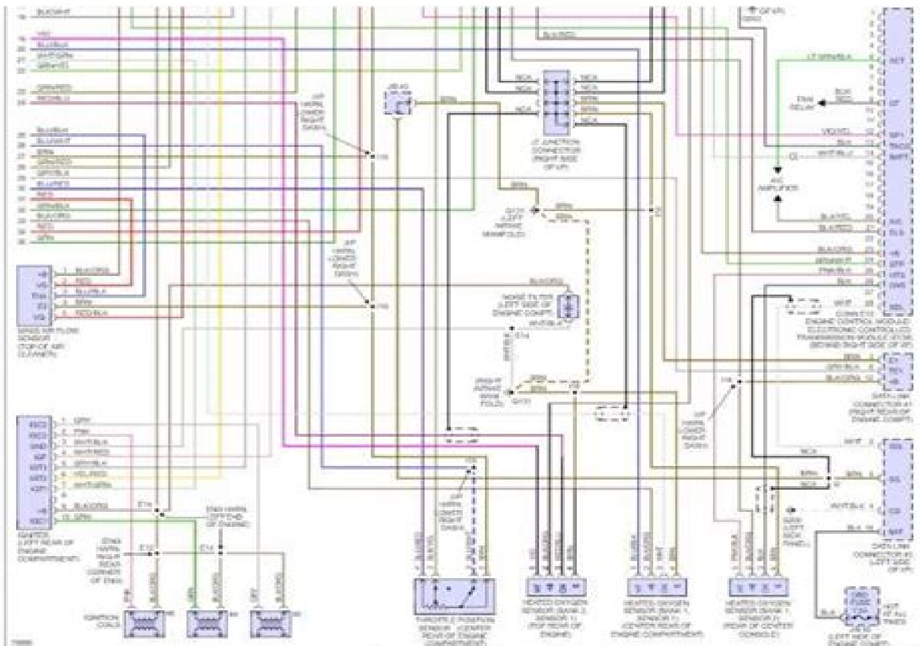
Fig 2 3.0L Engine Performance Circuits (2 of 2)
