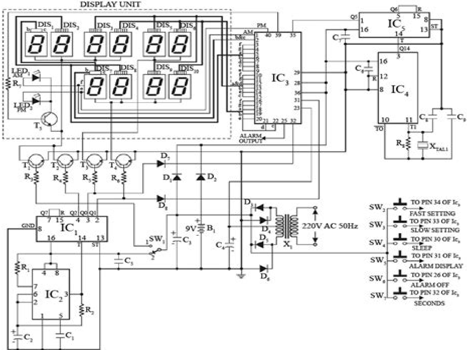
Figure 1: Circuit Diagram of Digital Clock with second and alarm display
