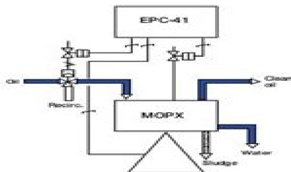
Fig. 2. Basic system-concept.
