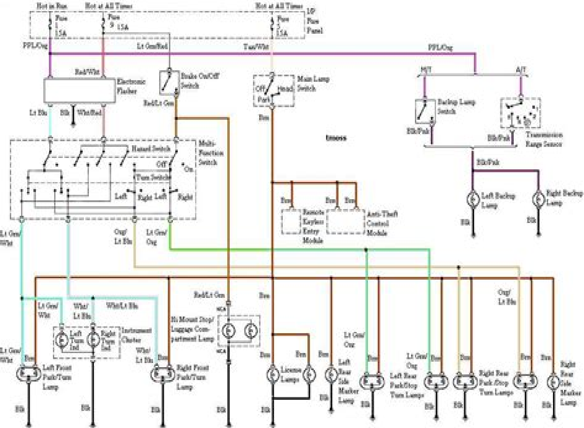
Typical Exterior Lighting System (w/o Headlamps & Fog Lamps)
