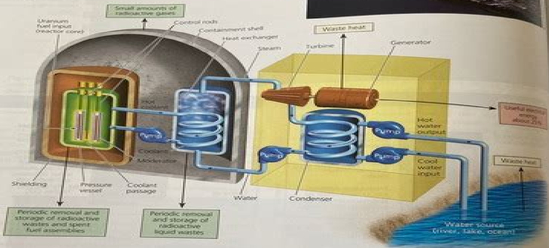
Figure 15-22 This water-cooled nuclear power plant, with a pressurized water reactor, produces intense heat that is used to convert water to steam, which spins a turbine that generates electricity. Question: How does this plant differ from the coal-burning plant in Figure 15-15?
