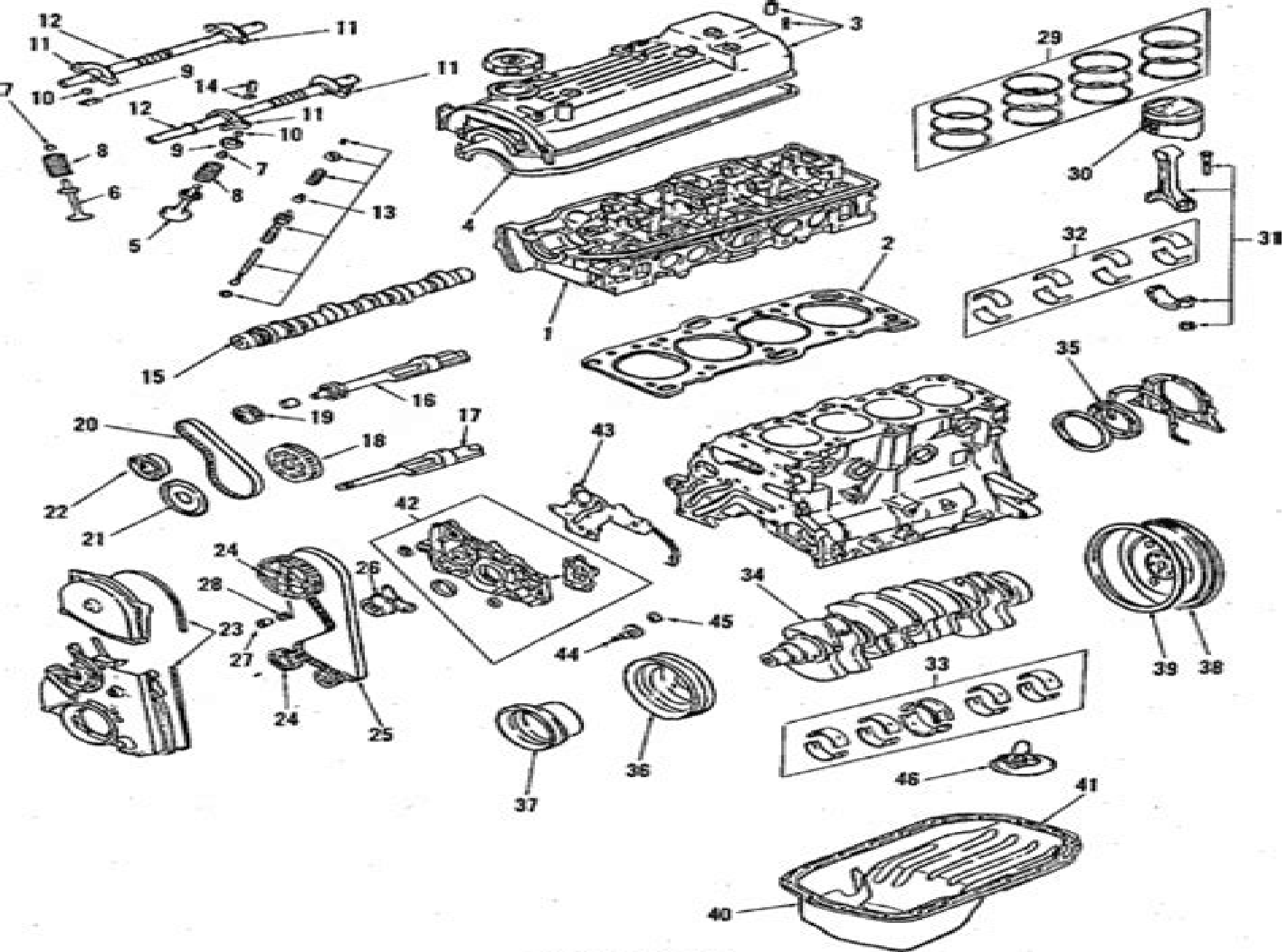
ENGINE 2000-2400
