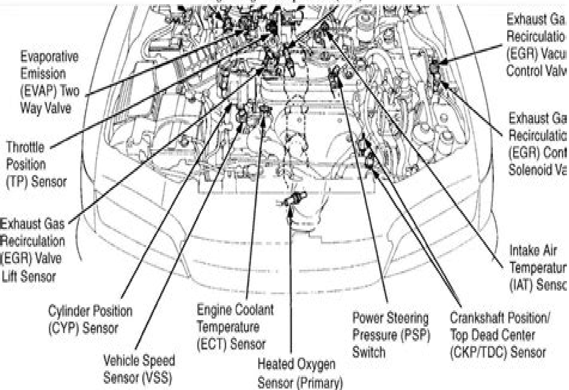
Fig. 4: Engine Compartment (2.2L)
