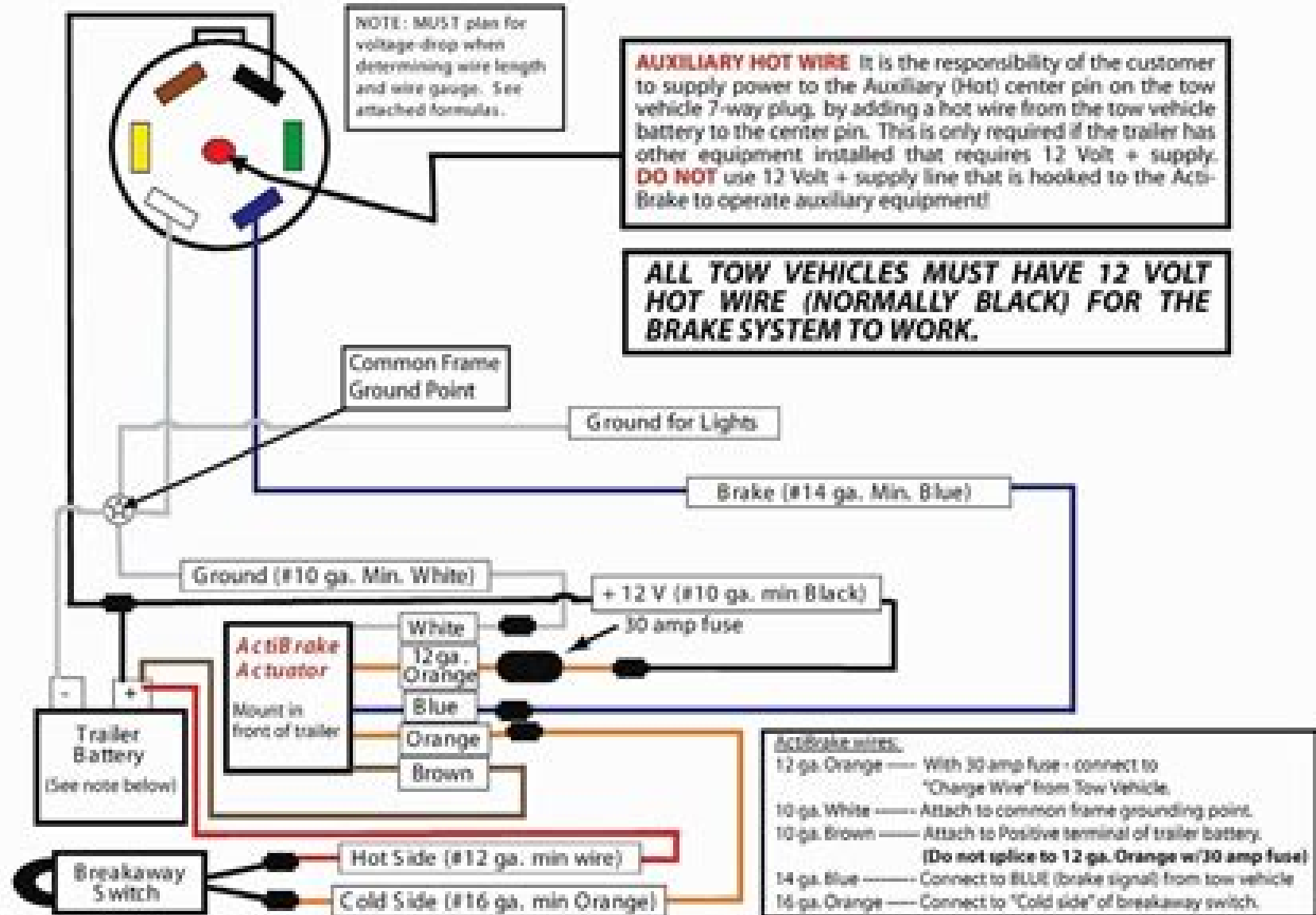
7-Way Trailer Plug (Rear View)
