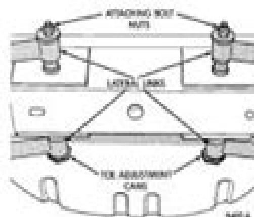
Fig. 5 Torquing Rear Lateral Link Attaching Bolts
