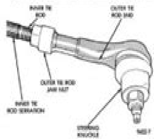
Fig. 7 Front Wheel Toe Adjustment
