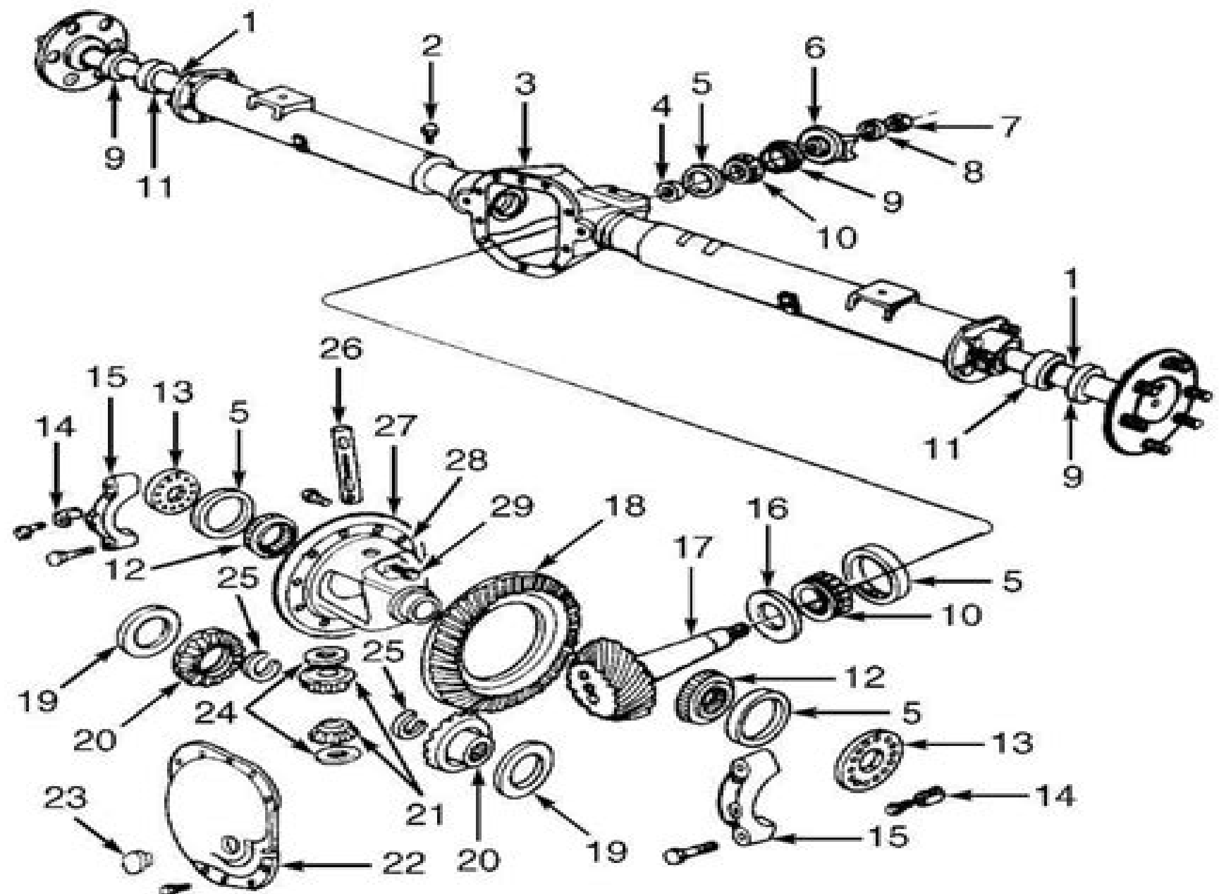
Fig. 1: Exploded View Of Drive Axle
