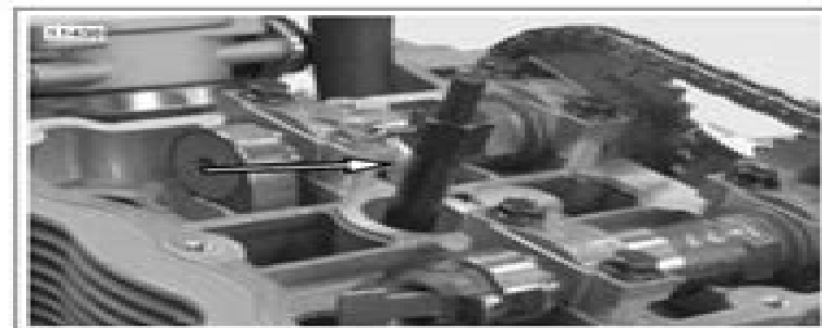
Figure 3-19. Top Dead Center Positioning Tool
