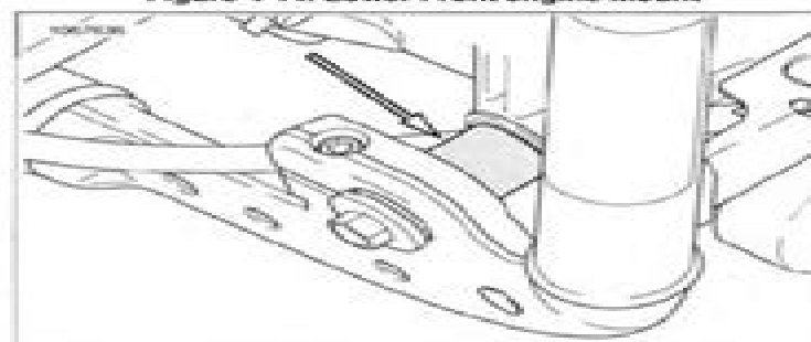
Figure 4-15. Spacer Installed Properly
