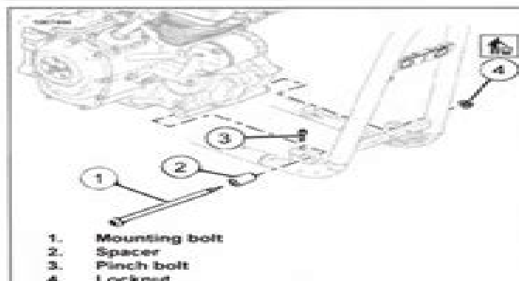
Figure 4-14. Lower Front engine Mount
