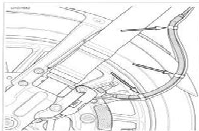
Figure 2-66. ABS Sensor Cable to Brake Hose Clips
