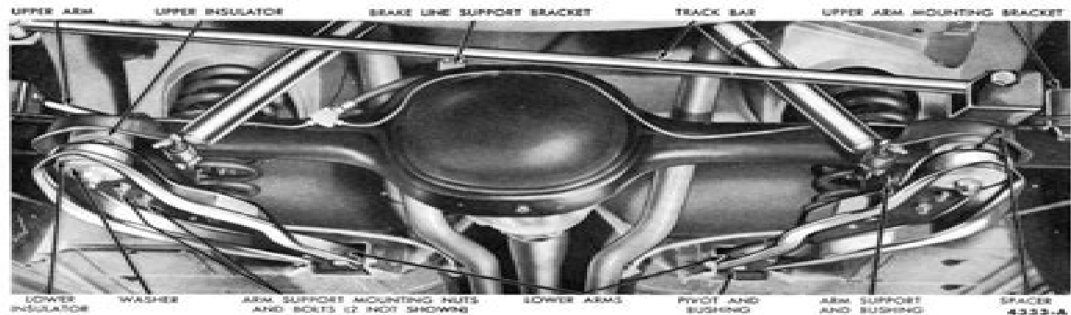
FIG. 14—Rear Suspension
