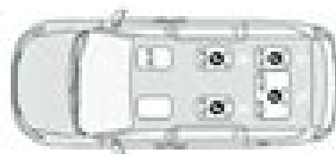
3 Passenger Side's Go Seating Automatic Locking Retractor (ALR) Locations
