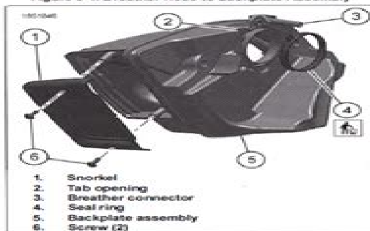
Figure 6-2. Backplate Assembly
