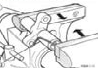
Fig. 95 Compressing Timing Belt Tensioner
