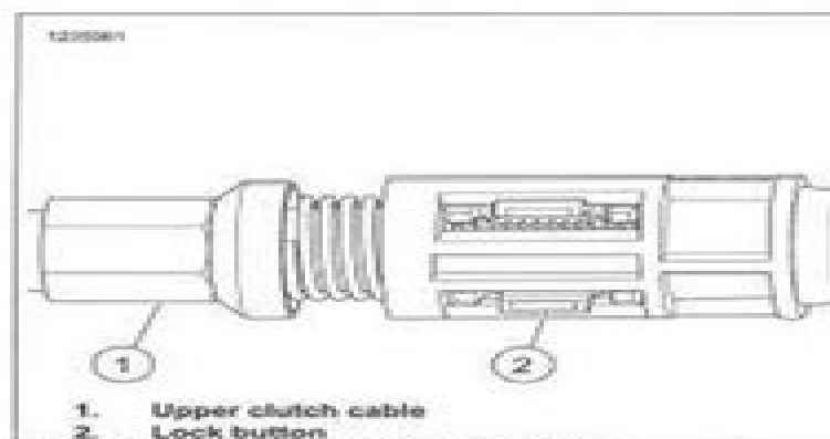
Figure 2-25. Compressed Upper Clutch Cable
