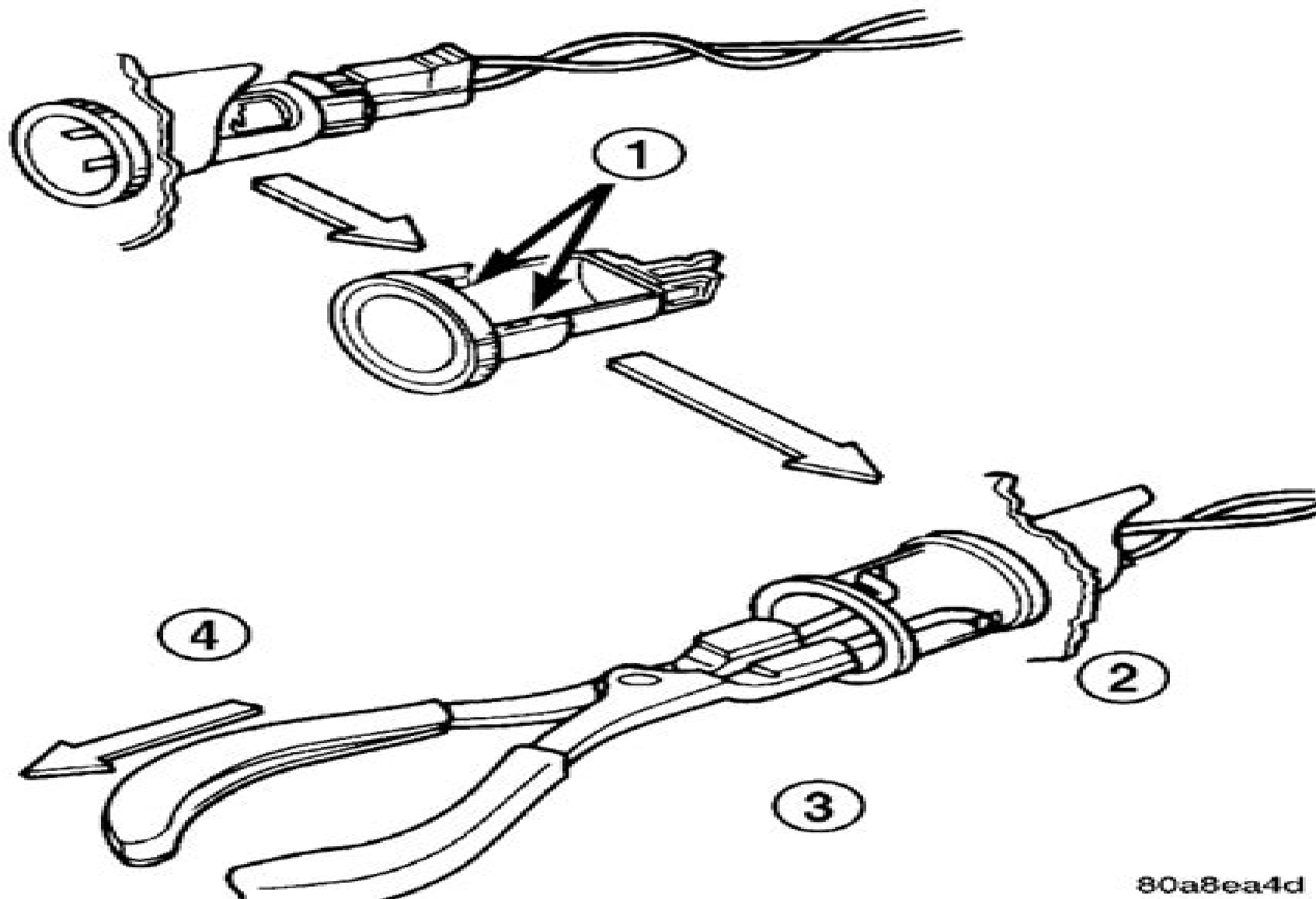
Fig 1: Removing/Installing Cigar Lighter/Power Outlet Base
