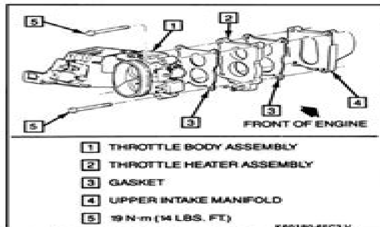
Figure 6E-C2-18 Throttle Body and Heater
