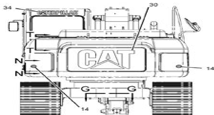
REAR VIEW
