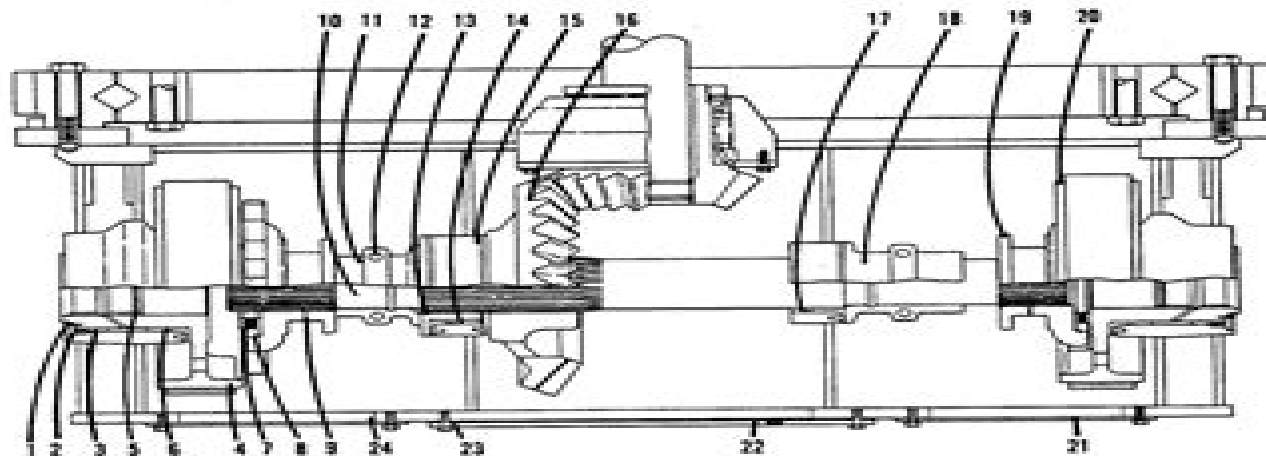
Fig. 1 Traction Shaft Assembly
