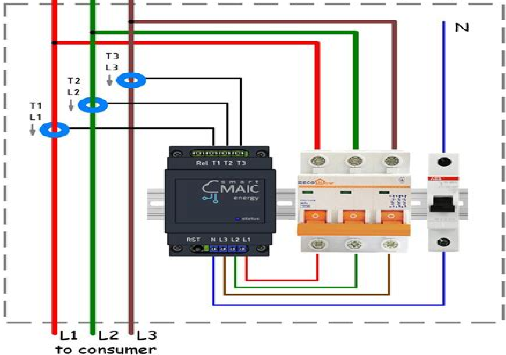
General connection diagram for smart-MAIC D103 in a 3-phase grid
